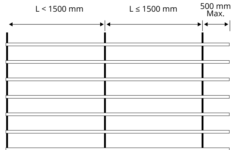
HORIZONTAL INSTALLATION
